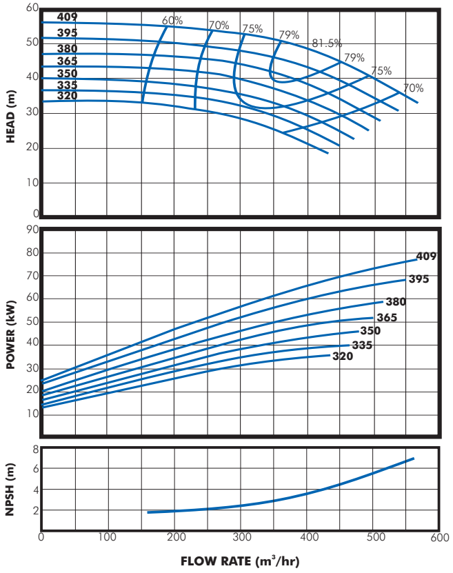
MODEL DE 150/40
