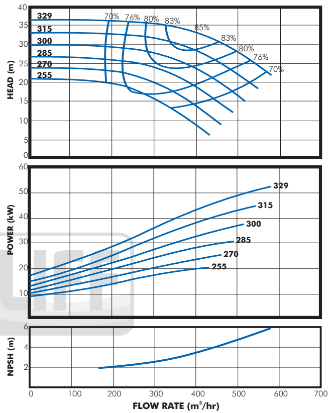
MODEL DE 150/32
