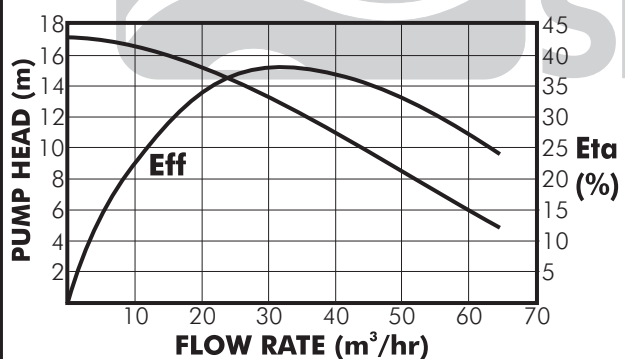
DW.65.27.03
